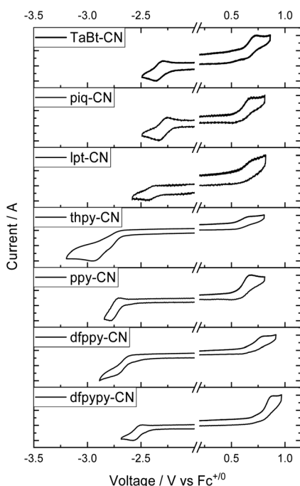
Fig. 3 Cyclic voltammograms of Ir(III)–CN complexes in CH 2 Cl 2 with n Bu 4 NPF 6 (0.1 M) as the supporting electrolyte. Conditions: scan rate: 100 mV s −1 ; glass-carbon, working electrode; Pt wire, counter electrode; saturated calomel electrode (SCE) in saturated KCl aqueous solution, and reference electrode.
