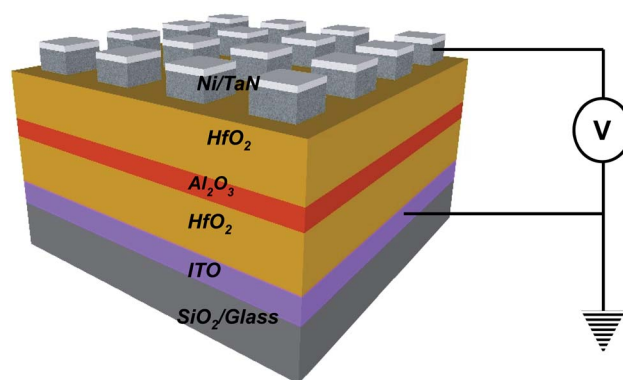
Fig. 1 Schematic of \text{Ni/TaN/HfO}_2/\text{Al}_2\text{O}_3/\text{HfO}_2/\text{ITO} RRAM device structure with TaN top and ITO bottom electrodes.
