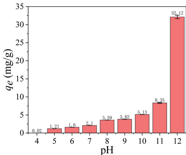
Fig. 5 Effect of pH on \text{Li}^+ adsorption capacity ( C_0 : 36 \text{ mmol L}^{-1} , T : 25^\circ\text{C} , t : 8 h).
