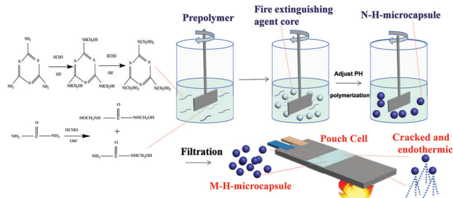
Fig. 1 Illustration of the synthesis of core-shell N-H-microcapsules and the action of the microcapsule on extinguishing lithium-ion battery fire.
