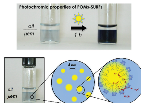
Fig. 15 (a) The partitioning of POM surfactants between the two phases of a WI microemulsion is easily achieved by irradiation with UV or even sunlight; (b) microemulsion is easily made of 5 nm diameter oil-containing micelles. Adapted from ref. 122 with permission from the Royal Society of Chemistry, copyright 2014.
