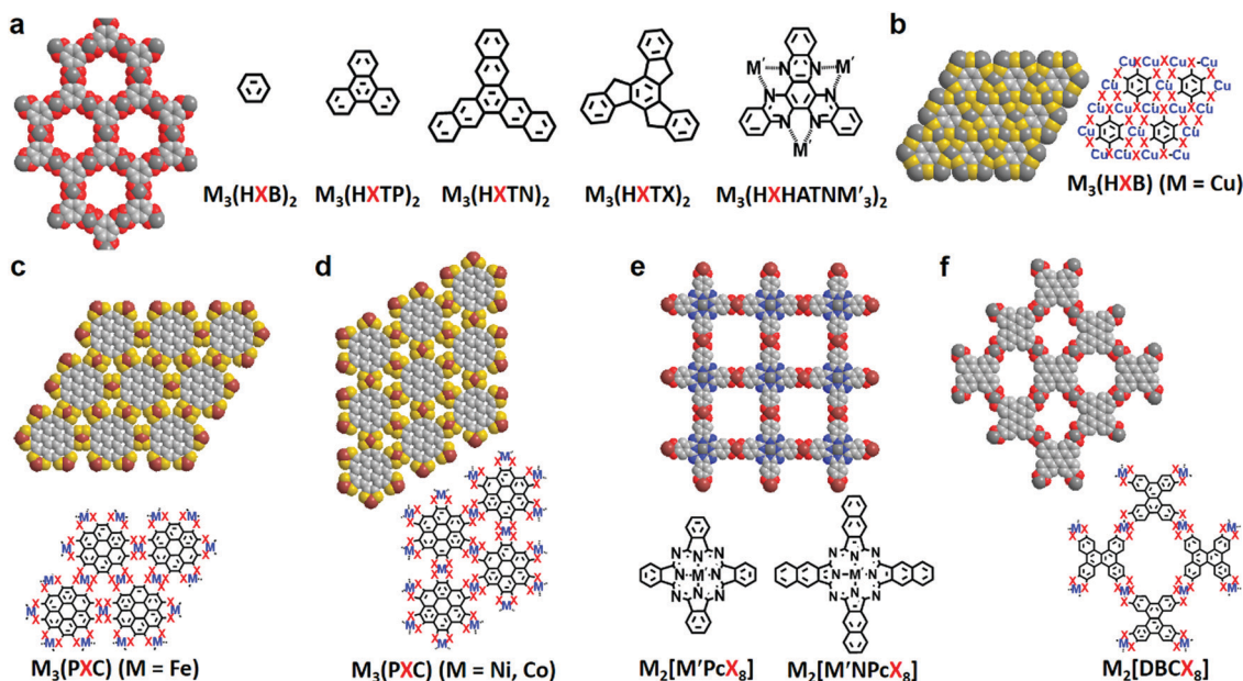
Fig. 2 Structure of various 2D c -MOFs. (a) 2D c -MOFs with honeycomb lattice. \text{M}_3(\text{HXB})_2 , \text{M}_3(\text{HXTTP})_2 , \text{M}_3(\text{HXTN})_2 , \text{M}_3(\text{HXTX})_2 , \text{M}_3(\text{HXHATNM}'_3)_2 . (b–d) Non-porous 2D c -MOFs. \text{M}_3(\text{HXB}) ( \text{M} = \text{Cu} ; \text{X} = \text{S}, \text{Se} ) and \text{M}_3(\text{PXC}) ( \text{M} = \text{Fe}, \text{Ni}, \text{Cu} ; \text{X} = \text{S} ). (e) 2D c -MOFs with square lattice. \text{M}_2[\text{M}'\text{PcX}_8] ( \text{M} = \text{Fe}, \text{Co}, \text{Ni}, \text{Cu}, \text{Zn} ; \text{M}' = \text{Fe}, \text{Ni}, \text{Cu}, \text{Zn} ; \text{X} = \text{O}, \text{NH} ) and \text{M}_2[\text{M}'\text{NPcX}_8] ( \text{M} = \text{Ni}, \text{Cu} ; \text{M}' = \text{Ni} ; \text{X} = \text{O} ). (f) Non-planar 2D c -MOF. \text{M}_2[\text{DBCX}_8] ( \text{M} = \text{Cu} ; \text{X} = \text{O} ).
