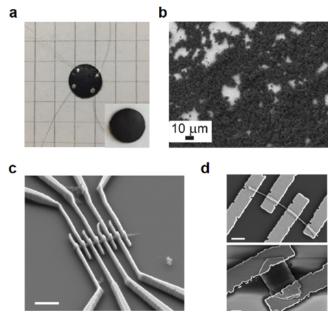
Fig. 16 Device integration of bulk 2D c -MOFs. (a) Pellet of 2D c -MOFs and device fabrication in the van der Pauw geometry. 55 Copyright 2020, Wiley-VCH. (b) SEM image of drop-cast Cu 3 (HITP) 2 on an indium-tin-oxide glass slide. Reproduced with permission ref. 28. Copyright 2015, Wiley-VCH. (c) SEM image of the fabricated device based on isolated single-crystalline Ni 3 (HITP) 2 nanorods. (d) SEM images of fabricated devices based on isolated single-crystalline Cu 3 (HITP) 2 nanorods (top) and nanoflakes (down). Reproduced with permission ref. 95. Copyright 2019, American Chemical Society.
