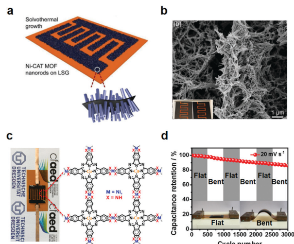
Fig. 27 2D c -MOFs based MSCs. (a and b) Illustration of LSG-supported Ni 9 (HHTP) 4 for MSC and its SEM image. Reproduced with permission ref. 100. Copyright 2019, Wiley-VCH. (c and d) Flexible MSC device based on Ni 2 [CuPc(NH) 8 ] nanosheets. 55 Copyright 2020, Wiley-VCH.
