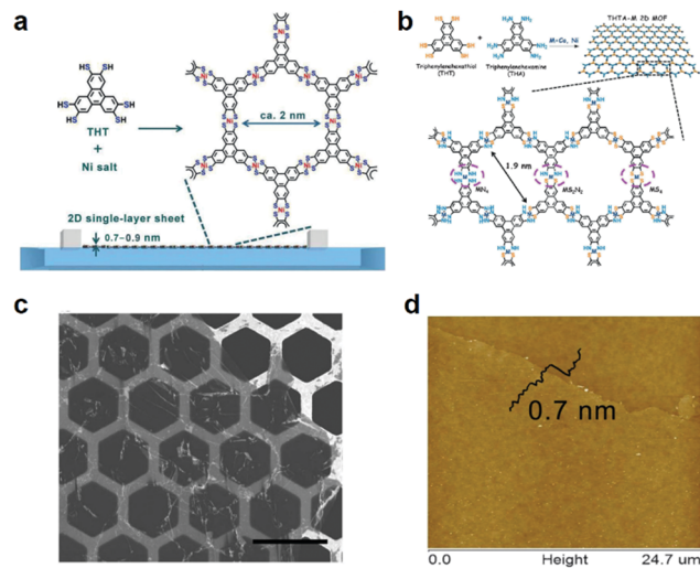
Fig. 15 Single-layer 2D c -MOFs synthesized through LB-assisted interfacial synthesis. (a and b) Schematic illustration of the synthesis of Ni 3 (HTTP) 2 and a Co 3 (HITP)(HTTP) 2D c -MOF comprising mixed ligands of HTTP and HATP. (c and d) SEM and AFM images of single-layer Ni 3 (HTTP) 2 . Reproduced with permissions. 45,61 Copyrights 2015 and 2017, Wiley-VCH.
