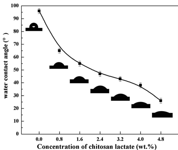
Fig. 4 Static contact angles of CL/PES composite NF membranes and PES UF membrane (CL concentration: 0 wt%).
