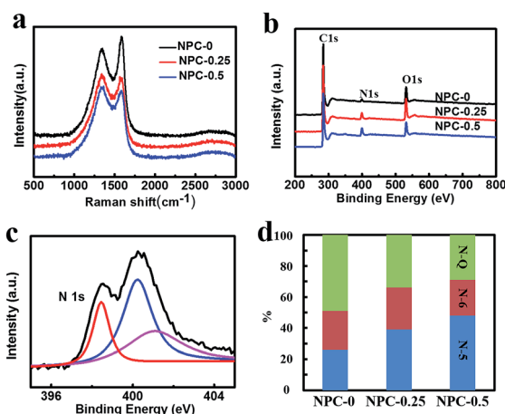
Fig. 4 Raman spectra of NPC-0, NPC-0.25 and NPC-0.5 (a). XPS spectra of NPC-0, NPC-0.25 and NPC-0.5 (b). High-resolution N 1s spectra of NPC-0.5 (c). The content of pyridine N (N-6), pyrrole N (N-5) and graphitization N (N-Q) of NPC-0, NPC-0.25 and NPC-0.5 (d).
