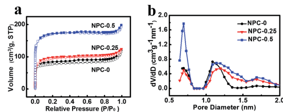
Fig. 3 \text{N}_2 absorption–desorption isotherm (a) and pore size distribution of NPC-0, NPC-0.25 and NPC-0.5 (b).
