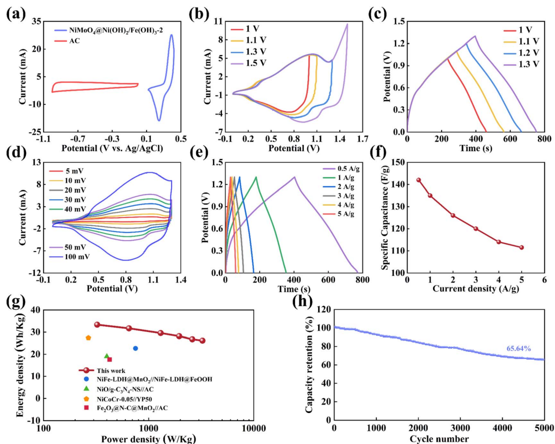
Fig. 9 (a) CV curves of the AC and \text{NiMoO}_4@\text{Ni}(\text{OH})_2/\text{Fe}(\text{OH})_3-2 electrodes at 50 \text{ mV s}^{-1} (b) CV curves under different potential ranges at 50 \text{ mV s}^{-1} , (c) GCD curves under different potential ranges at 0.5 \text{ A g}^{-1} , (d) CV curves at 5\text{--}100 \text{ mV s}^{-1} , (e) GCD curves at 0.5\text{--}5 \text{ A g}^{-1} , (f) specific capacitances at 0.5\text{--}5 \text{ A g}^{-1} , (g) Ragone plots of the power density and energy density, (h) cycling stability after 5000 cycles of the ASC.
