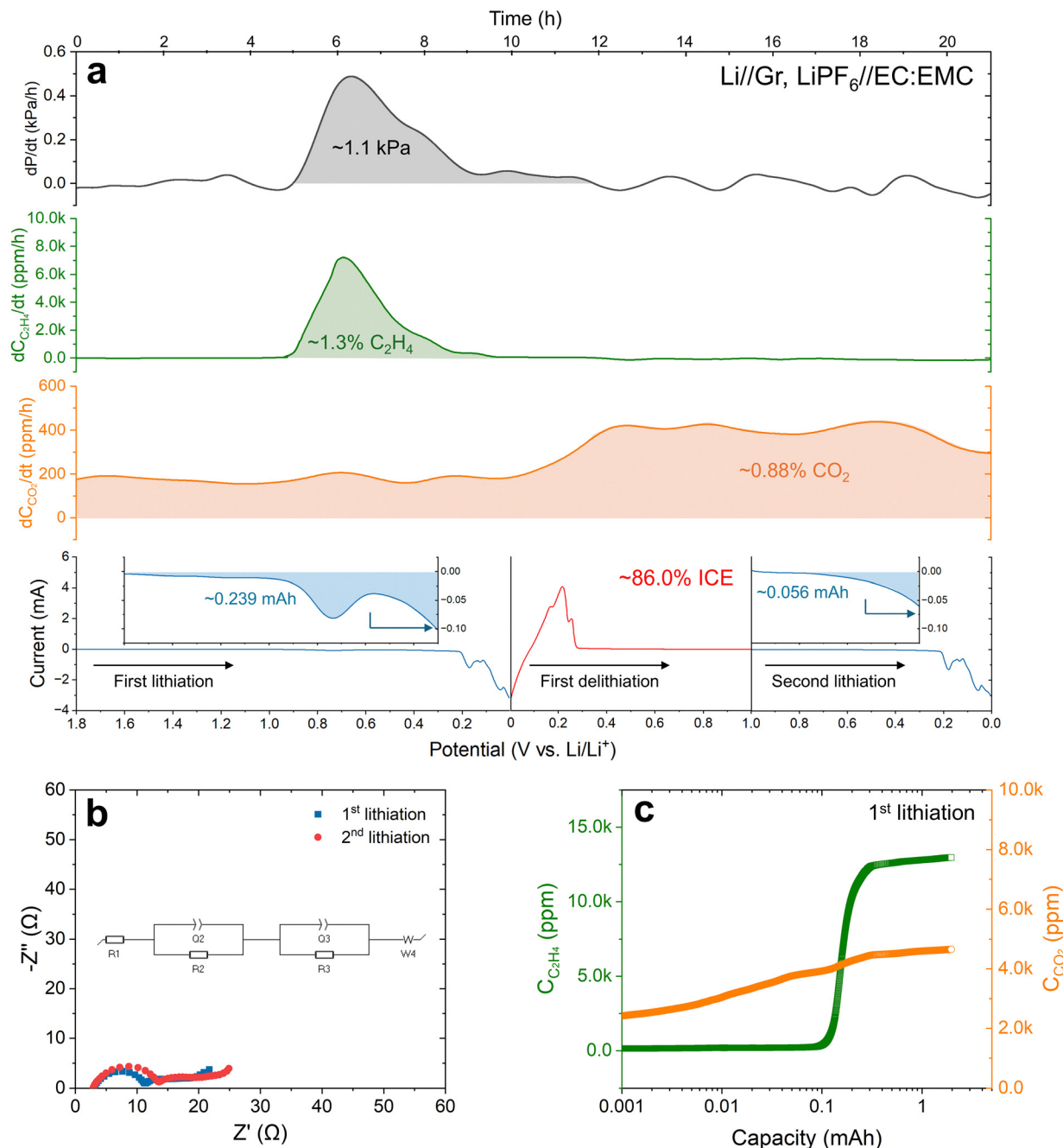
Fig. 5 Operando monitoring of gas evolution in the Li-graphite half-cell that undergoes cyclic voltammetry at a scan rate of 0.05 mV s^{-1} with 1 M LiPF_6 in EC : EMC 3 : 7 vol% as the electrolyte. (a) The obtained CV curves are plotted in conjunction with the change in concentrations of C_2H_4 , CO_2 , and in overall gas pressure. The detailed current variation from 1.8 V to 0.3 V vs. Li/Li^+ of the first lithiation and from 1 V to 0.3 V vs. Li/Li^+ of the second lithiation is provided in the insets by zooming in the y-axis. The blue shading of the first lithiation represents the electric charge consumed for the SEI formation and associated gas evolution. (b) The EIS spectra obtained after the initial and the second cathodic scan. (c) Evolution of C_2H_4 and CO_2 concentrations during the initial lithiation of graphite.
