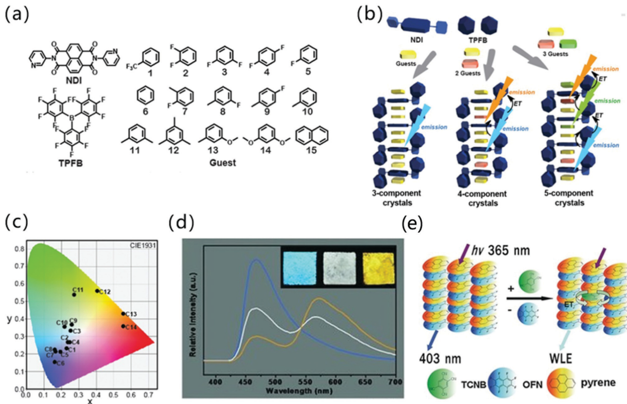
Fig. 6 (a) The structure of NDI, TPFB and aromatic guests composed of three-, four-, and five-component cocryystals. (b) Schematic illustration of three-, four-, and five-component crystalline materials. (c) Emission colors in the CIE 1931 chromaticity diagram of multi-component cocryystals. Reprinted with permission from ref. 46. Copyright 2019. The Royal Society of Chemistry. (d) Steady state emission spectra of mixed CT complex microtube films spin-coated on a quartz substrate at doping concentrations of 0 (blue), 0.015% (white), and 0.1% (orange) upon excitation with 365 nm. Insets show the corresponding photographs excited with a UV lamp (365 nm). The excitation wavelength is 365 nm. Reprinted with permission from ref. 48. Copyright © 2012 Wiley-VCH Verlag GmbH & Co. KGaA, Weinheim. (e) The energy transfer mechanism of pyrene-OFN and pyrene-TCNB. Reprinted with permission from ref. 49. Copyright © 2017 Wiley-VCH Verlag GmbH & Co. KGaA, Weinheim.
