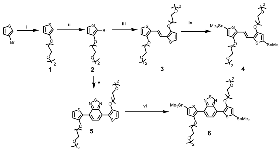
Scheme 1 The synthetic route of bis(trimethylstannyl) glycolated TVT, bis(trimethylstannyl) glycolated TBTT monomers. Reaction conditions: (i) t -BuOK, 2-(2-methoxyethoxy)ethanol, RT, then 100^\circ\text{C} ; (ii) NBS, THF/Hexane, 0^\circ\text{C} ; (iii) 2-bis(tributylstannyl)ethene, \text{Pd}_2(\text{dba})_3 , \text{P}(\text{o-tol})_3 , 100^\circ\text{C} ; (iv) n -BuLi, THF, -78^\circ\text{C} , \text{SnClMe}_3 , then RT; (v) 4,7-Bis(4,4,5,5-tetramethyl-1,3,2-dioxaborolan-2-yl)2,1,3-benzothiadiazole, \text{Pd}_2(\text{dba})_3 , \text{P}(\text{o-tol})_3 , tricaprylylmethylammonium chloride, aq. \text{K}_3\text{PO}_4 , toluene; (vi) n -BuLi, THF, -78^\circ\text{C} , \text{SnClMe}_3 , then RT.
