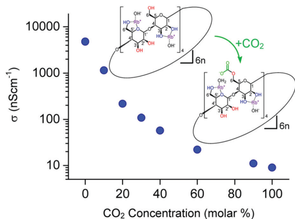
Fig. 6 Variations in the conductivity of CDMOF-2 upon \text{CO}_2 absorption/desorption cycles. 62
