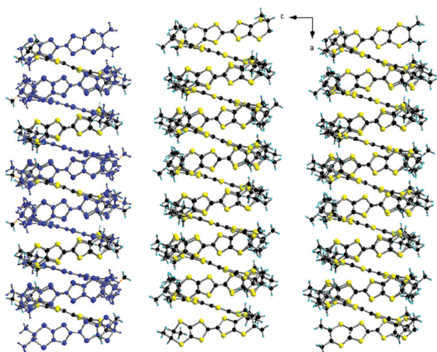
Fig. 3 Crystalline packing of [(S)\text{-}1]_9(\text{Mo}_6\text{O}_{19})_5(\text{CHCl}_3)_2 in the ac plane with a highlight of the two types of donors (left column, the asymmetric unit contains two donors 1^*\text{TTF} + \frac{1}{2}^*\text{TTF} ). Anions and solvent have been omitted.
