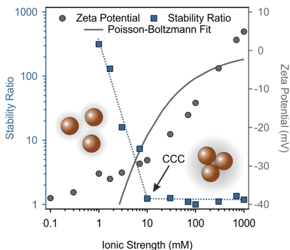
Fig. 5 Stability ratio (squares) and zeta potential (circles) values of \text{MnO}_2 NPs dispersions as a function of the ionic strength. The pH was kept at 9 in all samples. The dotted blue line only serves as eye guidance. The continuous grey line is the Poisson–Boltzmann fit.
