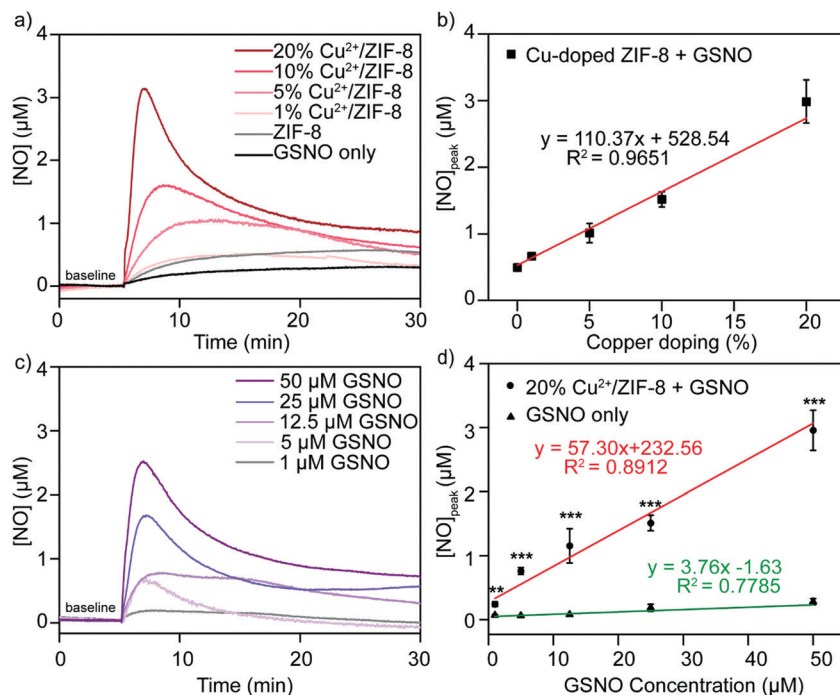
Fig. 4 (a) Representative NO generation profiles and (b) peak NO concentrations from GSNO (50 \mu\text{M} ) in the presence of \text{Cu}^{2+}/\text{ZIF-8} (0.1 \text{mg mL}^{-1} ) with different copper doping percentages (0–20%). (c) Representative NO generation profiles and (d) peak NO concentrations from catalytic decomposition of GSNO (1–50 \mu\text{M} ) by 20% \text{Cu}^{2+}/\text{ZIF-8} (0.1 \text{mg mL}^{-1} ). All reactions were performed in PBS at 37 ^{\circ}\text{C} . Values represent mean \pm standard deviation, n = 3 . Statistical significance relative to control tests was calculated, **p < 0.01 , ***p < 0.001 (one-way ANOVA followed by Tukey post hoc test).
