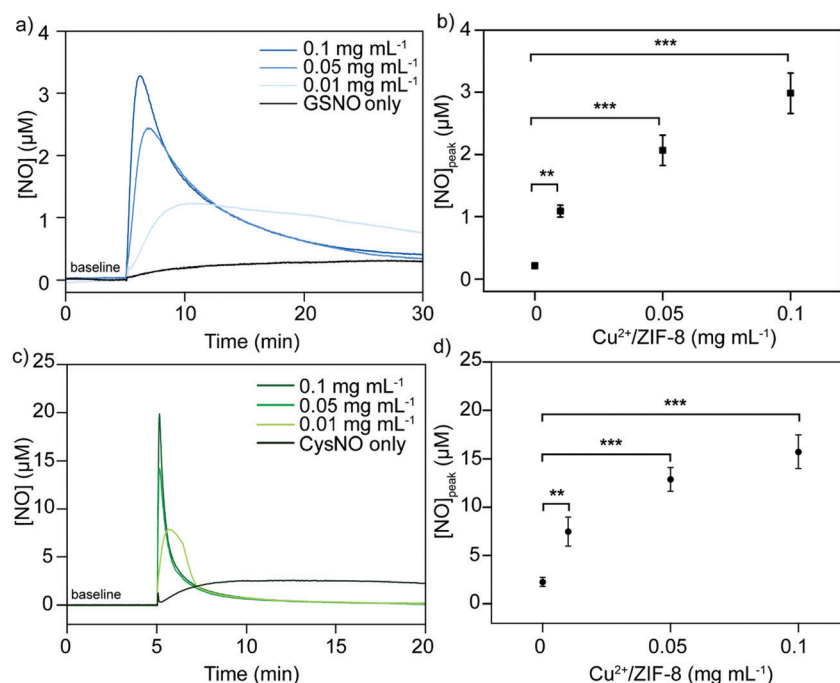
Fig. 5 (a) Representative NO generation curves and (b) peak NO concentrations from GSNO (50 \mu\text{M} ) by 20% \text{Cu}^{2+}/\text{ZIF-8} (0.01–0.1 \text{mg mL}^{-1} ). (c) Representative NO generation curves and (d) peak NO concentrations from CysNO (50 \mu\text{M} ) by 20% \text{Cu}^{2+}/\text{ZIF-8} (0.01–0.1 \text{mg mL}^{-1} ). Values represent mean \pm standard deviation, n = 3 . Statistical significance relative to control tests was calculated, **p < 0.01 , ***p < 0.001 (one-way ANOVA followed by Tukey post hoc test).
