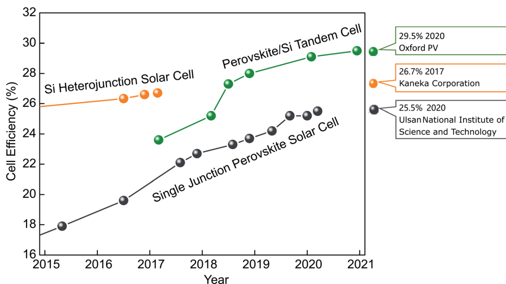
Fig. 3 Record efficiency evolution over the last five years for silicon heterojunction solar cell (26.7% by Kaneka Corporation), single junction perovskite solar cell (25.5% by Ulsan National Institute of Science and Technology), perovskite/Si tandem cell (29.5% by Oxford PV).
