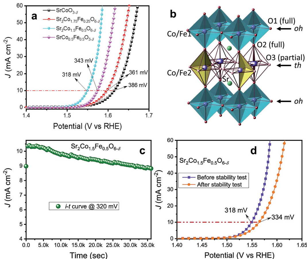
Fig. 7 (a) LSV plots of \text{SrCoO}_{3-\delta} , \text{Sr}_2\text{Co}_{1.75}\text{Fe}_{0.25}\text{O}_{6-\delta} , \text{Sr}_2\text{Co}_{1.5}\text{Fe}_{0.5}\text{O}_{6-\delta} and \text{SrCo}_{0.5}\text{Fe}_{0.5}\text{O}_{3-\delta} oxides; (b) structural model of the intermediate tetragonal phase containing a sequence of alternating octahedral (oh) and tetrahedral (th) layers (...oh-th-oh-th...), where only two randomly orientated tetrahedra are shown for clarity; (c) stability test of \text{Sr}_2\text{Co}_{1.5}\text{Fe}_{0.5}\text{O}_{6-\delta} oxide at 1.550 V vs. RHE for 10 h; (d) LSV plots of samples before and after the stability test. 57 Reproduced from ref. 57 with permission, © 2021 American Chemical Society.
