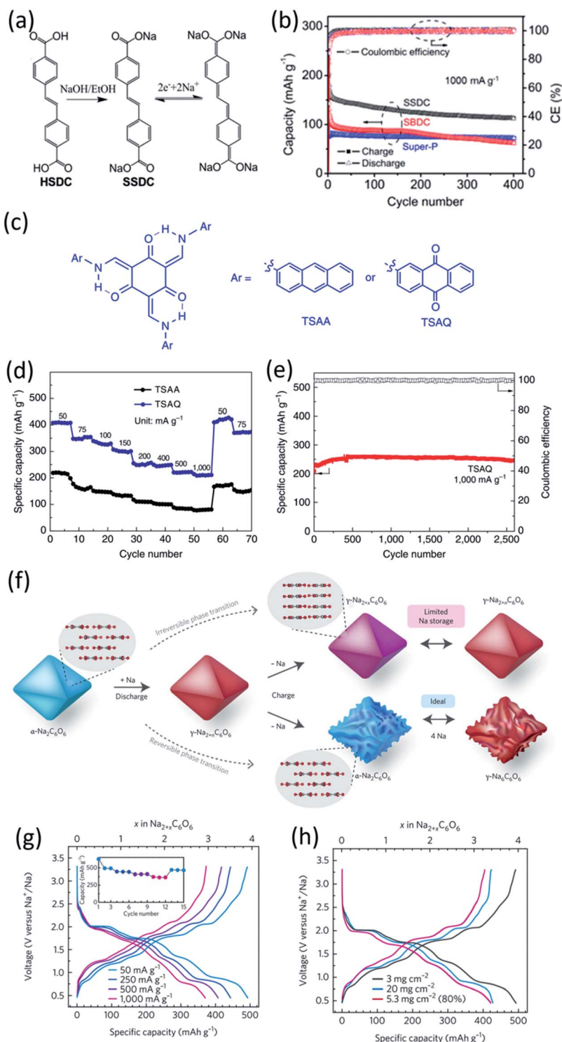
Fig. 2 (a) Schematic diagram for the synthesis and reversible Na-ion insertion/extraction mechanism of SSSDC. (b) Cyclability of SSSDC (black, the rate capability of Super-P (blue) and SBDC (red) are also presented for comparison) under a current density of 1\text{ A g}^{-1} . Reproduced with permission. 68 Copyright 2015 American Chemical Society. (c) Design of \beta -ketoenamine-linked compound-based organic electrode. Chemical structure of TSAA and TSAQ. (d) Rate performance of TSAA and TSAQ electrodes at various current densities. (e) Cycle performance and the corresponding Coulombic efficiency of TSAQ at a current density of 1,000\text{ mA g}^{-1} in the voltage range of 3–0.05 V for more than 2,500 cycles. Reproduced with permission. 69 Copyright 2016 Springer Nature. (f) A schematic of the proposed de/sodiation mechanism of Na_2C_6O_6 . During charging, the structural change from the \alpha - to the \gamma -phase is kinetically suppressed. This leads to a premature desodiation, which results in limited sodium storage in subsequent cycles. Nevertheless, the reversible phase transformation becomes possible by decreasing the particle size and selecting a proper electrolyte, which in turn facilitates ideal four-sodium storage in Na_2C_6O_6 . (g) Rate capability and corresponding cycle performance (inset) of Na_2C_6O_6 electrodes from 0.5–3.3 V. (h) Voltage profiles of Na_2C_6O_6 electrodes with high active content (80% Na_2C_6O_6 , 5.3\text{ mg cm}^{-2} ) and high mass loading (60% Na_2C_6O_6 , 20\text{ mg cm}^{-2} ) compared with the original condition (60% Na_2C_6O_6 , 3\text{ mg cm}^{-2} ). Reproduced with permission. 70 Copyright 2017 Macmillan Publishers Limited.
