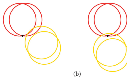
Fig. 5 Illustrations of “double” and “cusp” contacts shown in 2D as discussed in ref. 41. (a) Double contact: the yellow sphere is embedded into the red dimer so deeply that it contacts both red spheres. (b) Cusp contact: the yellow sphere contacts both red spheres by covering the cusp point (black point) of the red dimer.
