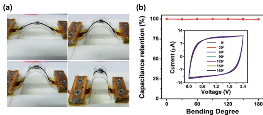
Fig. 10 (a) Photographs of the bending cycle of a flexible microsupercapacitor at different angles. (b) Capacitance retention graph across several bending angles. The inset shows the cyclic voltammograms of the device at those angles, showing a very stable performance. Reproduced with permission from ref. 163. Copyright 2019 Royal Society of Chemistry.
