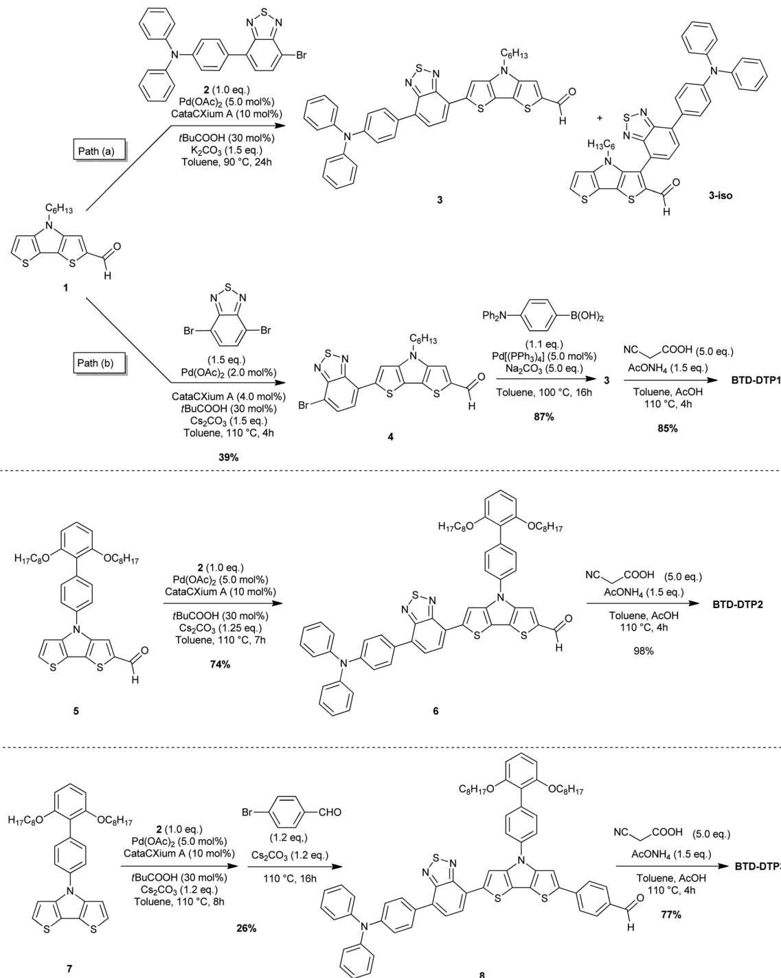
Scheme 1 Synthesis of the dyes BTD-DTP1–3.
