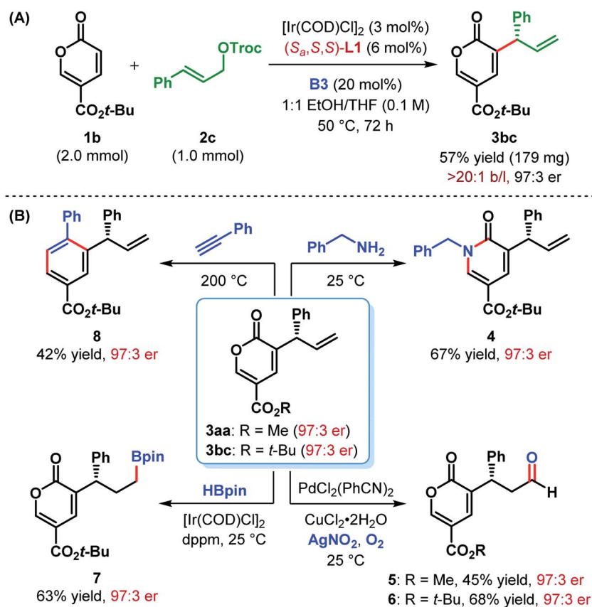
Scheme 3 (A) Scale-up of \alpha -C(sp 2 )-H allylic alkylation and (B) synthetic elaborations of \alpha -allyl-coumalates.
