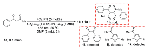
Scheme 4 Mechanistic studies.
