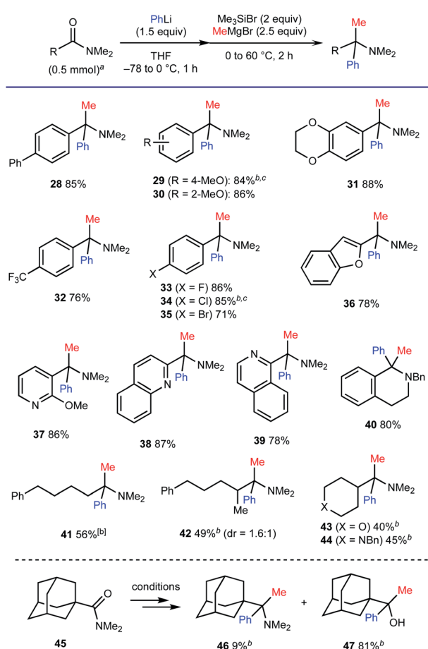
Scheme 6 Scope with respect to the carboxamides. a The reactions conditions: carboxamides (0.5 mmol), PhLi (1.5 equiv.) at -78 to 0^\circ\text{C} for 1 h, followed by Me_3SiBr (2 equiv.) and MeMgBr (2.5 equiv.) at 0^\circ\text{C} , then stirring at 60^\circ\text{C} for 2 h. Isolated yields were recorded. b 3 equiv. of MeMgBr was used. c After addition of MeMgBr , the reaction mixture was stirred at 60^\circ\text{C} for 3 h. Bn = benzyl.
