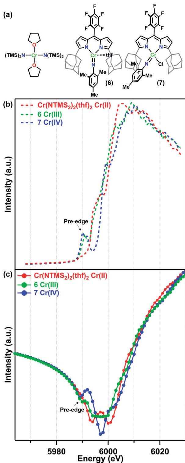
Fig. 2 (a) Reference molecules \text{Cr}(\text{NTMS}_2)_2(\text{thf})_2 , (\text{Ad}_{\text{LFS}})\text{Cr}(\text{NMes})(\text{thf}) (6), and (\text{Ad}_{\text{LFS}})\text{Cr}(\text{NMes})(\text{Cl}) (7) and their (b) fluorescence K-edge scans and (c) predicted f' spectra.
