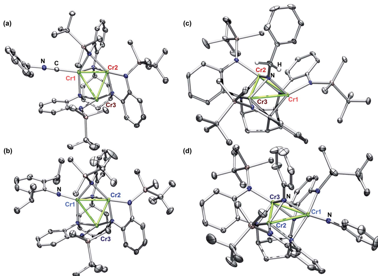
Fig. 1 Solid state molecular structures of (a) ( tb L)Cr 3 (CNBn) (4); (b) ( tb L)Cr 3 (NDipp) (2); (c) ( tb L)Cr 3 ( \mu^3 -NBn) (3); and (d) ( tb L)Cr 3 ( \mu^3 -NPh)(NPh) (5). Structures are presented with ellipsoids at 50% and some H atoms have been omitted for clarity (C gray, N blue, Si Pink, H white, Cr green).
