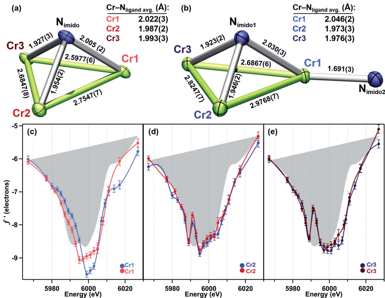
Fig. 5 Crystal structure cores with bond metrics (Å) indicated of (a) ({}^{\text{tbs}}\text{L})\text{Cr}_3(\mu^3\text{-NBn}) (3), and (b) ({}^{\text{tbs}}\text{L})\text{Cr}_3(\mu^3\text{-NPh})(\text{NPh}) (5). (c–e) Direct comparison of the anomalous scattering factor f' for (c) Cr1, (d) Cr2, and (e), Cr3 sites of 3 and 5 with the average f' for 4 shown in gray as a reference point for divalent chromium.
