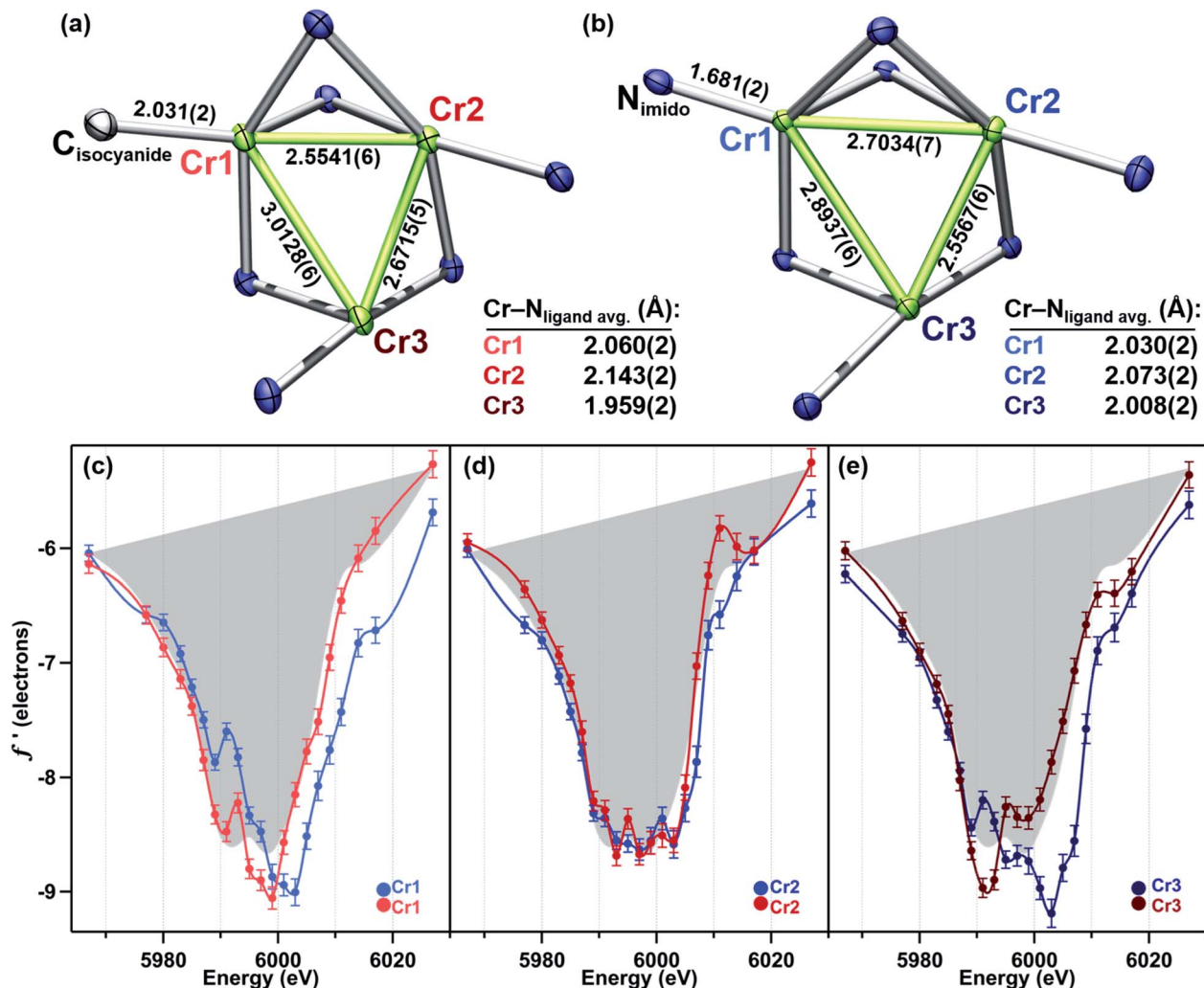
Fig. 4 Crystal structure cores with bond metrics (Å) indicated of (a) (^{t\text{Bu}}\text{L})\text{Cr}_3(\text{CNBn}) (4), and (b) (^{t\text{Bu}}\text{L})\text{Cr}_3(\text{NDipp}) (2). (c–e) Direct comparison of the anomalous scattering factor f' for (c) Cr1, (d) Cr2, and (e), Cr3 sites of 2 and 4 with the average f' for 4 shown in gray as a reference point for divalent chromium.
