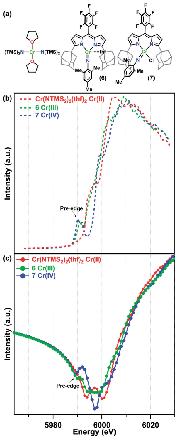
Fig. 2 (a) Reference molecules \text{Cr}(\text{NTMS}_2)_2(\text{thf})_2 , (\text{Ad}_{\text{LFS}})\text{Cr}(\text{NMe})_3(\text{thf}) (6), and (\text{Ad}_{\text{LFS}})\text{Cr}(\text{NMe})_3(\text{Cl}) (7) and their (b) fluorescence K-edge scans and (c) predicted f' spectra.
