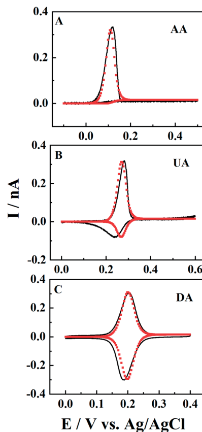
Fig. 7 The experimental (black solid lines) and simulated (red points) voltammograms of AA, UA and DA in CNPs. The concentration is 0.5 mM with 10 mM PBS (pH 7.4) buffer. Fitted value: a = 50 nm, d = 800a , \tan \theta = 0.15 , and v = 0.1 \text{ V s}^{-1} . k_c > 0.8 , k_c = 0.2 , and k_c < 0.01 \text{ s}^{-1} and E_0 = 0.11/0.27/0.2 \text{ V} for AA, UA and DA.
