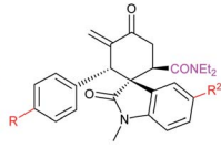
Scheme 4 Asymmetric diastereodivergent [4 + 2] annulation by tuning the catalytic system or substrate.
