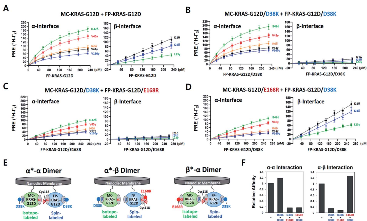
Fig. 2 KRAS-G12D \alpha\text{-}\alpha dimers associate in a specific manner while \alpha\text{-}\beta association is non-specific. (A) PRE rates of ILV ^{13}\text{C} -methyl probes in the \alpha and \beta interfaces of MC-KRAS-G12D as a function of the concentration of FP-KRAS-G12D bearing a TEMPO spin label at Cys118 in the \alpha interface. (B–D) PRE rates obtained with three combinations of interface mutants of KRAS-G12D, as indicated. (E) Schematic of the molecular configurations of the KRAS-G12D dimers favored by the interface mutants in panels B–D ( \alpha^*\text{-}\alpha , \alpha^*\text{-}\beta , or \beta^*\text{-}\alpha ): green; isotopically labelled MC-KRAS-G12D: blue; spin labelled FP-KRAS-G12D. The isotopically labeled interfaces exhibiting PRE effects are indicated with an asterisk in each label. (F) Relative affinities for \alpha\text{-}\alpha and \alpha\text{-}\beta interactions of KRAS-G12D and the engineered mutants indicated derived from data in panels A–D. Relative affinities ( 1/K_D ) are normalized to the interaction between MC-KRAS-G12D and FP-KRAS-G12D in panel A.
