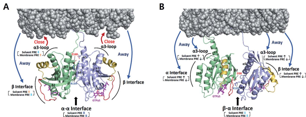
Fig. 3 Dimerization-induced changes in the solvent and membrane PRE (based on \Delta^1\text{H-}\Gamma_{2,\text{di-mono}}/\Gamma_{2,\text{mono}} values in Fig. S14b†) for each dimer state mapped onto the NMR-driven structure of the \alpha - \alpha (A) or \alpha - \beta dimer (B) of KRAS-G12D on the membrane. Dimerization-induced changes in proximity to the membrane are represented by red (closer) and blue (further) arrows. The side chains of key residues for each dimerization interface are depicted. Switch I and II regions are colored red and yellow, respectively.
