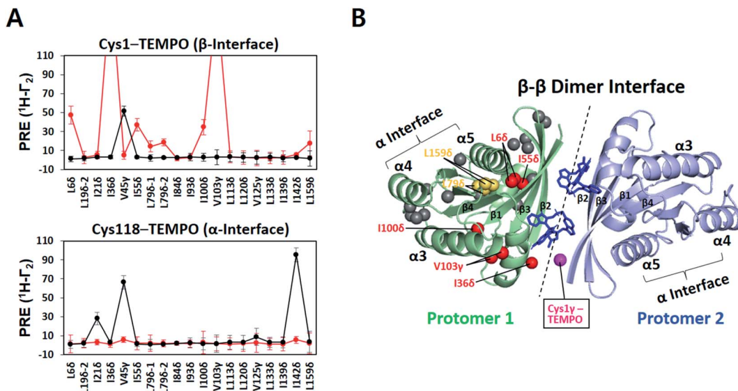
Fig. 4 KRAS inhibitor BI-2852 induces KRAS-G12D dimerization through a \beta - \beta interface on the membrane surface. (A) Intermolecular ^1\text{H} - ^1\text{T}_2 PRE rates for ILV ^{13}\text{C} -methyls of MC-KRAS-G12D in the presence of equimolar FP-KRAS-G12D bearing a TEMPO spin label at Cys1 in the \beta interface or Cys118 in the \alpha interface before (black lines) and after addition of BI-2852 (red lines, KRAS-G12D : BI-2852 molar ratio 1 : 1). (B) MC-KRAS-G12D probes exhibiting PRE effects from Cys1-TEMPO-tagged FP-KRAS-G12D upon addition of BI-2852 mapped onto a NMR-driven structure of a BI-2852-stabilized KRAS-G12D \beta - \beta dimer. One protomer is depicted with ILV ^{13}\text{C} -methyl probes coloured according to PRE exhibited in red, yellow, and gray, representing strong ( >30\text{ s}^{-1} ), moderate ( >10\text{ s}^{-1} ), and negligible PRE, respectively. Two BI-2852 molecules at the \beta - \beta dimer interface are shown in blue. In the opposing protomer, the Cys1 gamma position, the TEMPO conjugation site, is shown in purple.
