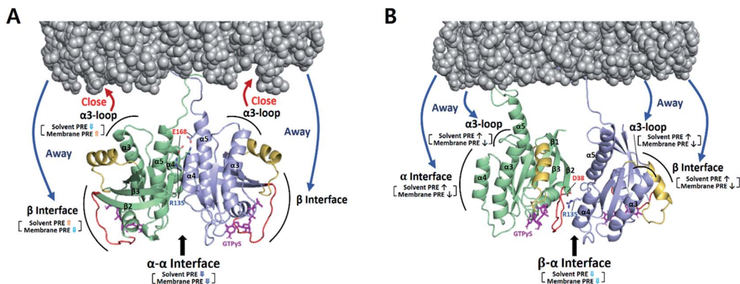
Fig. 3 Dimerization-induced changes in the solvent and membrane PRE (based on \Delta^1\text{H}-\Gamma_{2,\text{di-mono}}/\text{H}-\Gamma_{2,\text{mono}} values in Fig. S14b†) for each dimer state mapped onto the NMR-driven structure of the \alpha - \alpha (A) or \alpha - \beta dimer (B) of KRAS-G12D on the membrane. Dimerization-induced changes in proximity to the membrane are represented by red (closer) and blue (further) arrows. The side chains of key residues for each dimerization interface are depicted. Switch I and II regions are colored red and yellow, respectively.
