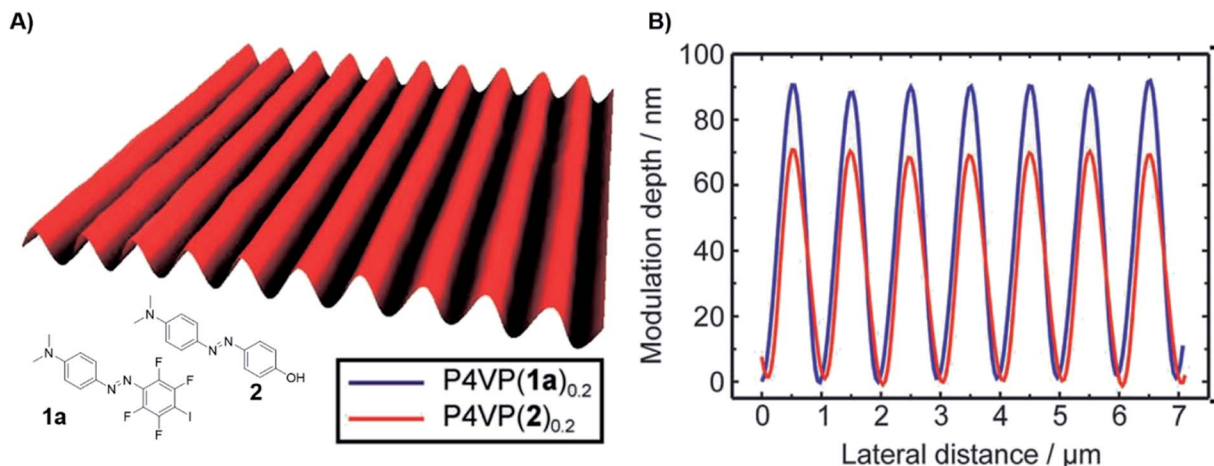
Fig. 9 (A) AFM surface relief of the surface relief grating film composed of P4VP and azobenzene containing XB-donor 1a, (B) modulation depth of the HB (2, red) and XB (1a, blue) films (reprinted with permission from ref. 41).
