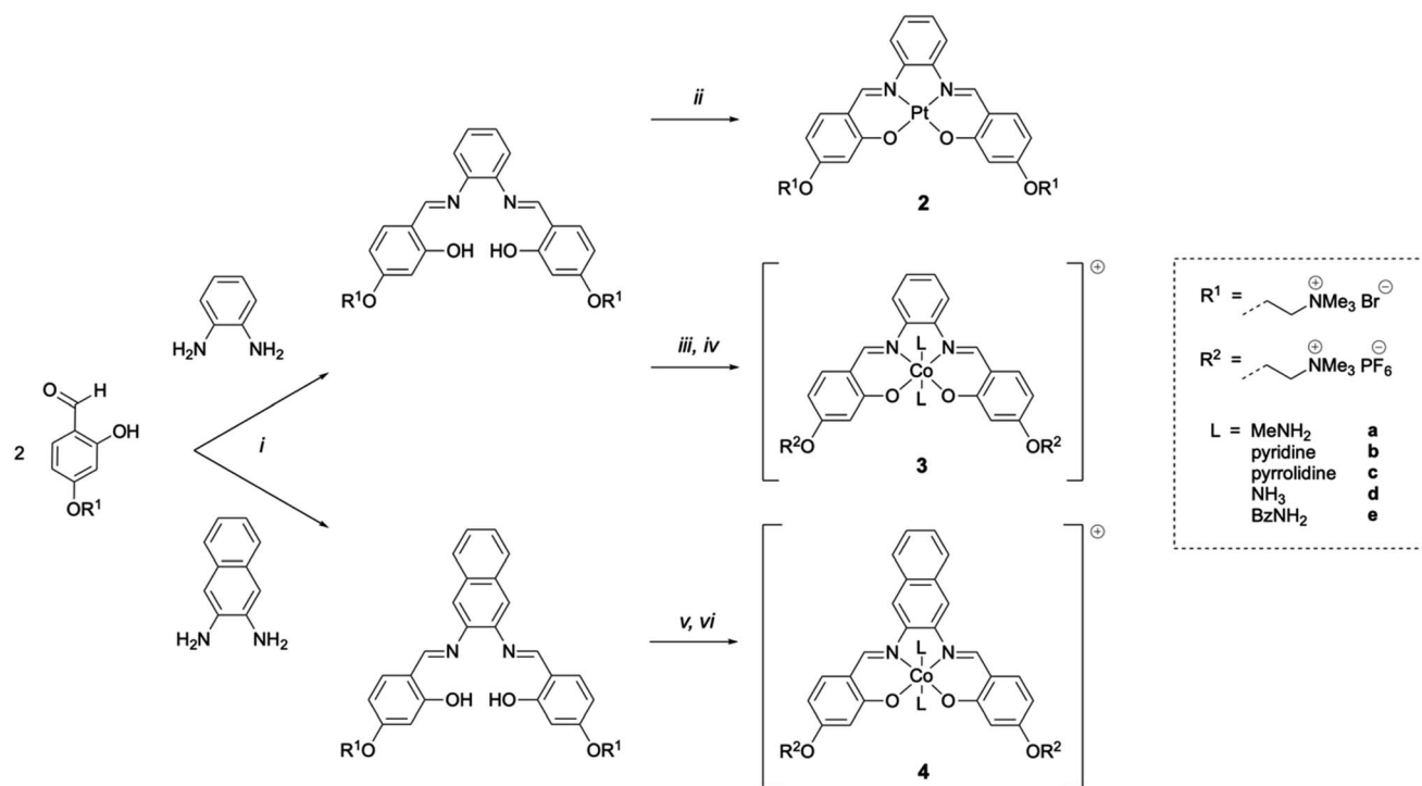
Scheme 1 Synthesis routes to complexes 2 , 3a–3e and 4a–4e . [i] EtOH, reflux, 5 h, N_2 ; [ii] K_2PtCl_4 , DMSO, 65 °C, 18 h, N_2 ; [iii, iv] Co(OAc)_2 \cdot 4H_2O , MeOH, r.t., 1 h, N_2 ; [iv] 10 eq. axial ligand L, aq. sat. NH_4PF_6 , MeOH, r.t., 3 h, air; [v] Co(OAc)_2 \cdot 4H_2O , MeOH, r.t., 1 min, air; [vi] 10 eq. axial ligand L, aq. sat. NH_4PF_6 , MeOH, r.t., 5 h, air.
