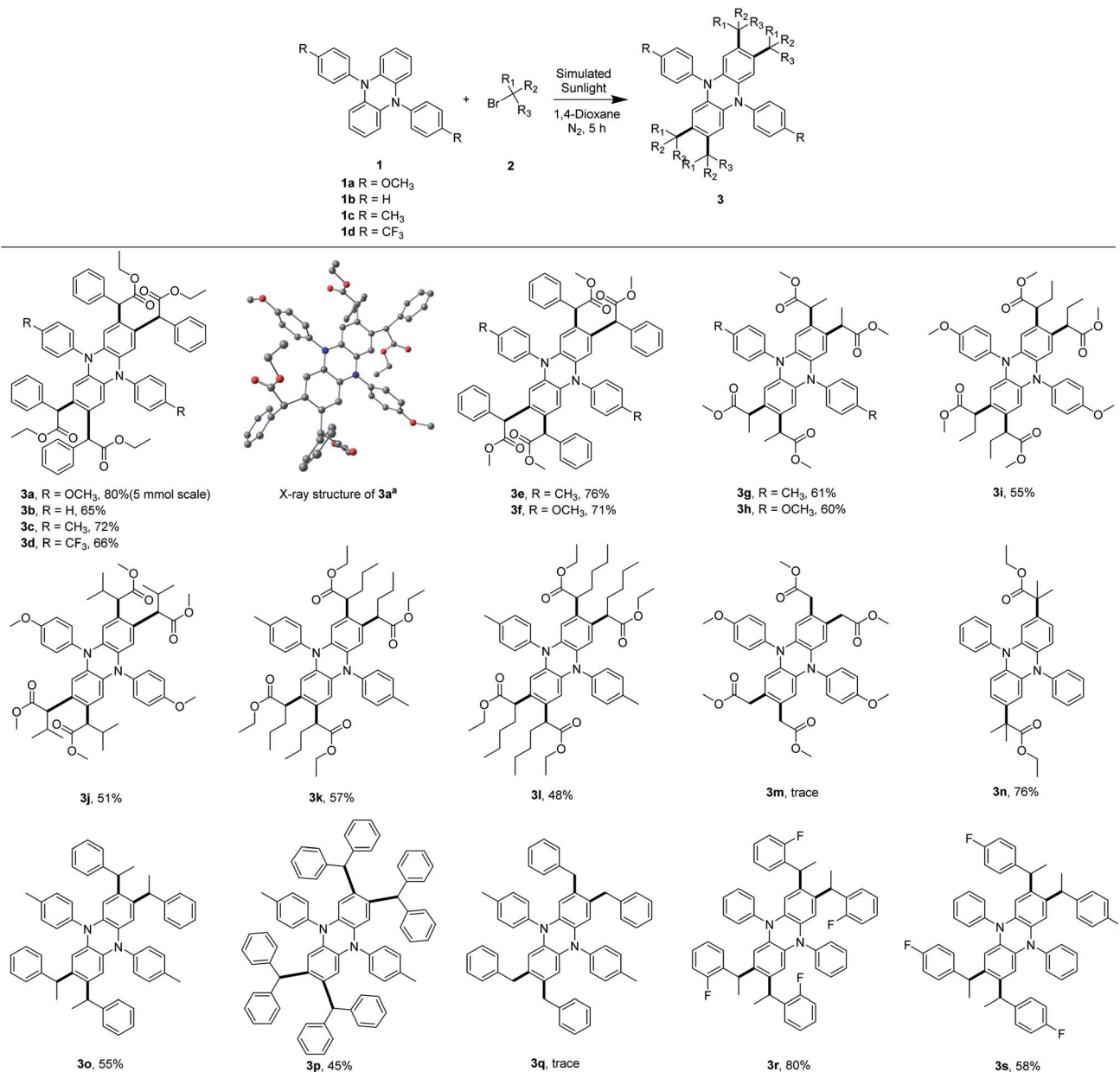
Fig. 2 Substrate scope of core modification of dihydrophenazines. Reaction conditions: a reaction mixture of 1 (100 mg, 1.0 equiv.) and 2 (100 equiv.) in 1,4-dioxane (10 mL) was irradiated with a 300 W simulated sunshine bulb at room temperature under N 2 for 5 h; isolated yields are shown. a Structure of 3a obtained by X-ray crystallography; H atoms are omitted for clarity. Color code, C: black, O: red, and N: dark blue (CCDC 2043491†).
