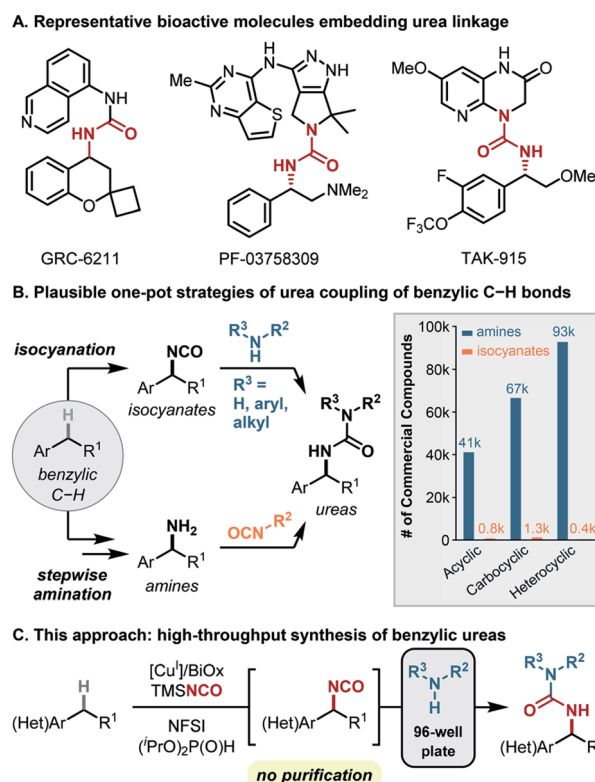
Fig. 1 Copper-catalyzed benzylic C(sp 3 )–H isocyanation/amine coupling. (A) Drug candidates embedding benzylic urea. (B) Two possible one-pot synthetic approaches toward ureas from benzylic C–H substrates. (C) Strategy for high-throughput synthesis of ureas. NFSI, N -fluorobenzenesulfonimide; BiOx, 2,2′-bis(oxazoline); TMSNCO, (trimethylsilyl)isocyanate.
