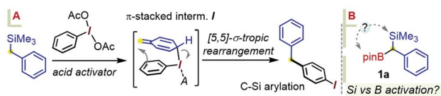
Scheme 3 (A) A precedent in the iodane-guided C–Si arylation of benzylsilanes with \lambda^3 -iodanes (Hyatt et al. and Shafir et al. ), 2018–19. (B) Potential selectivity dilemma in the analogous arylation of 1a .
