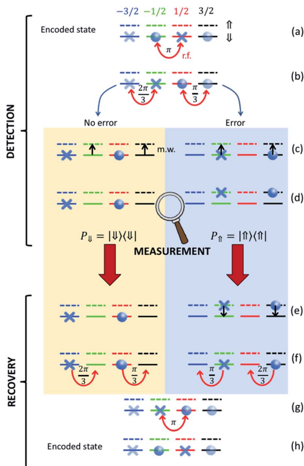
Fig. 7 Correction procedure on nuclear spin 3/2. Starting from a generic superposition of the code words (eqn (3a) and (3b)) we first (a and b) apply r.f. pulses targeting the transitions indicated by curved red arrows (with the indicated angles). This sequence brings no error (yellow box) and error (blue) cases to orthogonal states, which then follow a different evolution when subject to the same pulse sequence. In particular, the electronic ancilla is excited by two simultaneous \pi m.w. pulses (black arrows) only if the nuclear spin is in |m_{I_z} = -1/2\rangle and |m_{I_z} = 3/2\rangle (c). Then a measurement of the electronic qubit (insensitive to the nuclear spin) projects either into the \downarrow or into the \uparrow manifold (d). Only in the latter case the electronic spin is de-excited (e) and, finally, a different sequence of r.f. recovery pulses is applied, depending on the measurement outcome (f and g). The encoded state is finally recovered (h).
