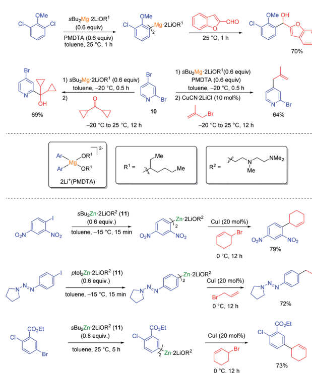
Scheme 4 Halogen/magnesium and zinc exchanges using the exchange reagents s\text{Bu}_2\text{Mg}\cdot 2\text{LiOR}^1 , s\text{Bu}_2\text{Zn}\cdot 2\text{LiOR}^2 or p\text{Tol}_2\text{Zn}\cdot 2\text{LiOR}^2 ( 11 ).
