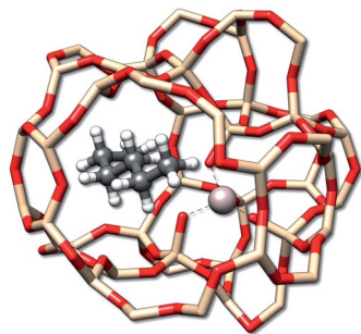
Fig. 10 The n -hexane molecule adsorbed by a H-ZSM-5 zeolite. Hydrogen atoms used for the saturation of the zeolite have been omitted for better visibility.
