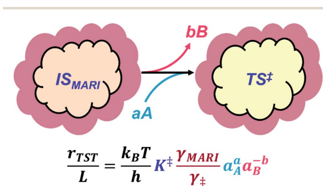
Fig. 1 A general reaction scheme illustrating the quantitative effects of clustering and solvation on catalytic rate expressions: (i) clustering, represented as the orange/yellow inner clouds, reflects the structure and molecularity of the transition state (TS) and most abundant reaction intermediates (MARI) that comprise the initial state (IS), and (ii) solvation by the surroundings, represented by the dark red outer clouds. A and B are generic fluid-phase species, accompanied by their stoichiometric coefficients ( a , b ), that require addition or removal from the cluster en route from the IS to the TS in the apparent rate-determining step.
