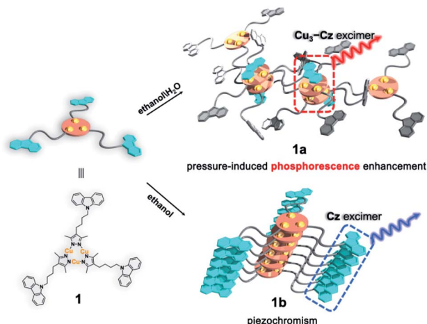
Scheme 1 A schematic representation showing the molecular stacking of two crystalline polymorphs 1a and 1b , and the formation of the \text{Cu}_3\text{Pz}_3 CTC \text{Cz}-\text{Cu}_3-\text{Cu}_3-\text{Cz} excimer and carbazole (Cz) excimer with an increase in pressure.
