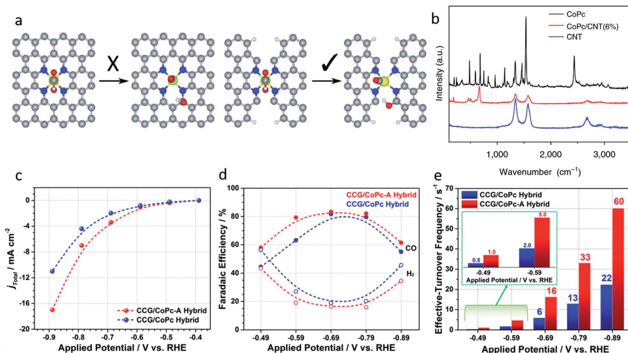
Fig. 6 (a) Ni-N 4 -C 10 sites (left) are inactive for the *COOH dissociation reaction, Ni-N 2+2 -C 8 sites are active because of the dangling bonds on the adjacent C atoms. Reproduced from ref. 82 with permission from the Royal Society of Chemistry, copyright 2019. (b) Raman spectra of CoPc, the CoPc/CNT(6%) hybrid, and CNTs. Reproduced from ref. 31 with permission from Springer Nature, copyright 2017. (c) Total current density, (d) faradaic efficiencies, and (e) effective turnover frequencies of CCG/CoPc-A and CCG/CoPc hybrids. Reproduced from ref. 85 with permission from the American Chemical Society, copyright 2019.
