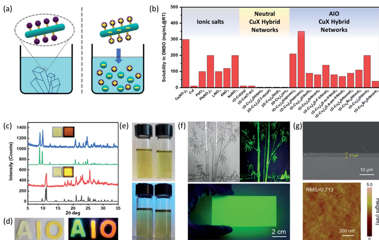
Fig. 3 (a) Structure similarity and solubility difference of charge-neutral 1D-CuI(L) (Left, Insoluble) and 1D-AIO-(Cu m X m+2 ) 2 (right, soluble) compounds. (b) Solubility data for common inorganic salts (left), neutral CuI(L) networks (middle) and 1D-AIO-(Cu m X m+2 ) 2 compounds (right). (c) PXRD patterns of thin films of AIO-type extended networks (red and blue) and corresponding simulated patterns from single crystal data (black and green). Inset: optical images of thin films of 1D-μ 1 -Cu 6 I 8 (btdmpm) 2 and 1D-μ 2 -Cu 4 I 6 (5-m-bttmp) 2 under daylight (left) and 365 nm UV light (right). (d) Selected 1D-AIO compounds coated on soft fabric (left: under daylight; right: under ultraviolet light source). (e) Optical images of 200 mg 1D-μ 1 -Cu 6 I 8 (btdmpm) 2 (left) and 1D-μ 2 -Cu 4 I 6 (5-m-bttmp) 2 (right) dissolved in 3 ml DMSO under day light (top) and 365 nm UV light (bottom). (f) A picture painted by the 0D-Cu 4 I 6 (pr-ted) 2 /PVP ink under natural light (top left) and 365 nm ultraviolet light (top right), respectively and a large-area film deposited on glass substrate by a doctor-blade coating process (bottom). (g) Cross-sectional SEM image (top) and AFM image (bottom) of the as-fabricated 0D-Cu 4 I 6 (pr-ted) 2 /PVP film. (a), (c)–(e) are reproduced with permission from ref. 30. Copyright 2020, American Chemical Society. (f)–(g) are reproduced with permission from ref. 36. Copyright 2020, American Chemical Society.
