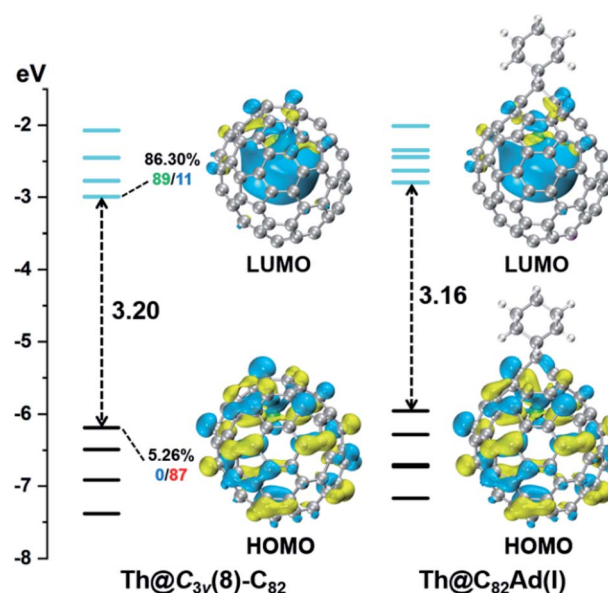
Fig. 9 Frontier molecular orbitals of Th@C 3v (8)-C 82 and Th@C 3v (8)-C 82 Ad(I) (occupied: black; unoccupied: cyan). For selected orbitals, the participation (%) of the Th AOs is first given, followed by two numbers showing the % contribution of the Th-5f (red), -6d (blue), or -7s (green) AOs to this metal hybrid orbital.
