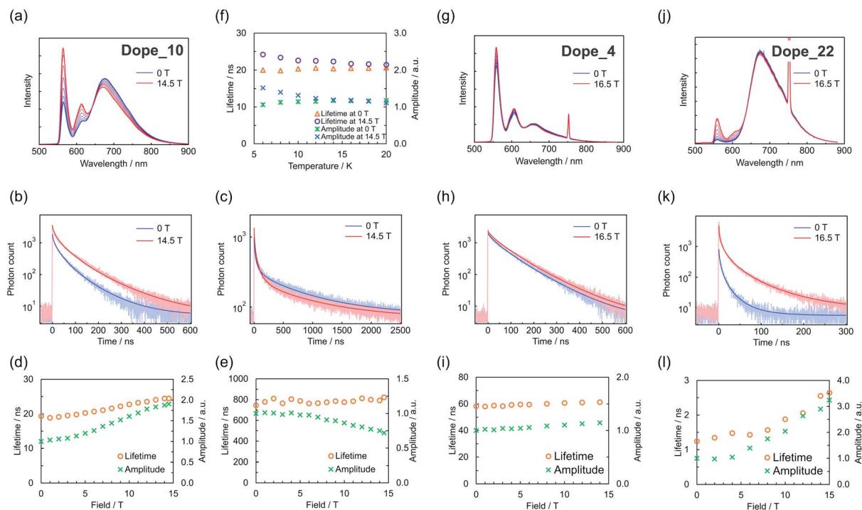
Fig. 2 (a–e) Emission spectra of Dope_10 at 4.2 K under magnetic fields of 0–14.5 T at 563 nm (a), emission decays and corresponding fits at 4.2 K under magnetic fields of 0 and 14.5 T at 563 nm (b) and 674 nm (c), and magnetic field dependences of lifetimes and amplitudes at 4.2 K at 563 nm (d; \beta = 0.59 ) and 674 nm (e; \beta = 0.88 ). (f) Temperature dependences of lifetimes and amplitudes at 563 nm under magnetic fields of 0 and 14.5 T ( \beta = 0.59 ). (g–i) Emission spectra of Dope_4 at 4.2 K under magnetic fields of 0–16.5 T (g), emission decays and corresponding fits at 4.2 K under magnetic fields of 0 and 16.5 T (h), and magnetic field dependences of lifetimes and amplitudes at 4.2 K (i) ( \beta = 0.78 ). (j–l) Equivalent results as in (g–i) for Dope_22 ( \beta = 0.41 ). Peaks at 750 nm are due to the excitation laser light ( \lambda_{\text{ex}} = 375 nm).
