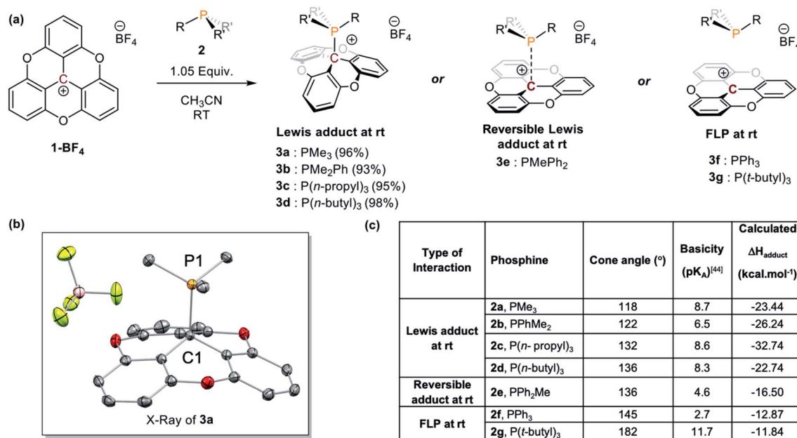
Scheme 1 (a) Reactivity of phosphines ( 2a–2g ) towards \text{TOTA}^+ . (b) ORTEP of the X-ray structure of 3a . Hydrogen atoms and counter ion are omitted for clarity. (c) Summary of cone angle, Lewis basicity, and DFT calculated \Delta H_{\text{adduct}} (enthalpy of adduct formation relative to free TOTA and phosphine) for phosphines 2a–2g .
