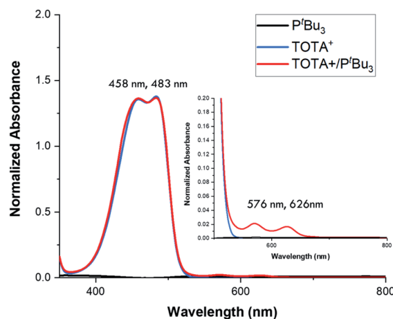
Fig. 3 Normalized UV-vis spectra of \text{TOTA}^+ (blue trace, 1 \times 10^{-5} \text{ M} in \text{CH}_2\text{Cl}_2 ), \text{P}^t\text{Bu}_3 (black trace, 1 \times 10^{-5} \text{ M} in \text{CH}_2\text{Cl}_2 ), and a 1 : 1 mixture of \text{P}^t\text{Bu}_3/\text{TOTA}^+ (red trace, both substrates 1 \times 10^{-5} \text{ M} in \text{CH}_2\text{Cl}_2 ).
