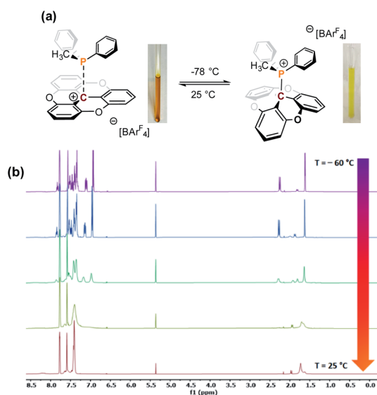
Fig. 2 (a) Reversible Lewis adduct formation between \text{TOTA}^+ and \text{PPh}_2\text{Me} . (b) Variable temperature (VT) 500 MHz ^1\text{H} NMR spectra of \text{TOTA}^+ (12 mg, 0.01 mmol) and \text{PPh}_2\text{Me} (4.2 mg, 0.02 mmol) in \text{CD}_2\text{Cl}_2 indicating formation of Lewis adduct at -60^\circ\text{C} .
