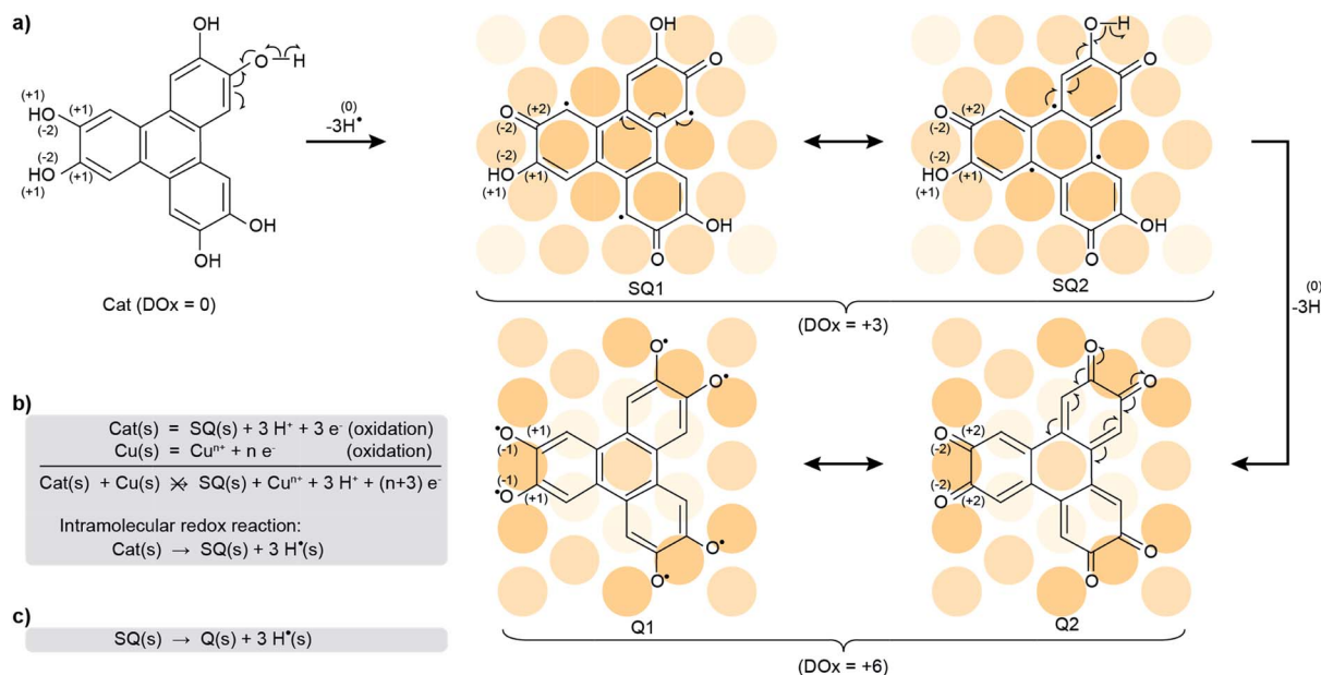
Scheme 1 Oxidation of a catechol into a semiquinone and a quinone. (a) Two-step oxidation (with departure of three hydrogen radicals, -3\text{H}^* , at each step) of the HHTP molecule, a catechol (Cat), into a semiquinone, of which two mesomers are shown (SQ1, SQ2), and a quinone, of which two mesomers are shown (Q1, Q2). The mesomers each correspond to a distinct charge distribution. Only one third of the charge reorganisation processes are shown. The surface Cu atoms are sketched with orange balls, with the darkest orange shades used to highlight those atoms forming stronger bonds with the molecules. The global degree of oxidation (DOx) is indicated for each molecule, and the individual DOxs of relevant H atoms and one third of the C atoms linked to O atoms, and of these O atoms, are specified in parenthesis. (b) The simultaneous oxidation of both the catechol and the Cu metal would yield the semiquinone and Cu ions, an impossible process. Instead, an intramolecular redox reaction transforms the HHTP molecule into the semiquinone molecule. (c) A similar kind of reaction transforms the semiquinone into the quinone molecule.
