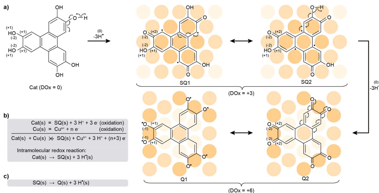
Scheme 1 Oxidation of a catechol into a semiquinone and a quinone. (a) Two-step oxidation (with departure of three hydrogen radicals, -3\text{H}^{\cdot} , at each step) of the HHTP molecule, a catechol (Cat), into a semiquinone, of which two mesomers are shown (SQ1, SQ2), and a quinone, of which two mesomers are shown (Q1, Q2). The mesomers each correspond to a distinct charge distribution. Only one third of the charge reorganisation processes are shown. The surface Cu atoms are sketched with orange balls, with the darkest orange shades used to highlight those atoms forming stronger bonds with the molecules. The global degree of oxidation (DOx) is indicated for each molecule, and the individual DOxs of relevant H atoms and one third of the C atoms linked to O atoms, and of these O atoms, are specified in parenthesis. (b) The simultaneous oxidation of both the catechol and the Cu metal would yield the semiquinone and Cu ions, an impossible process. Instead, an intramolecular redox reaction transforms the HHTP molecule into the semiquinone molecule. (c) A similar kind of reaction transforms the semiquinone into the quinone molecule.
