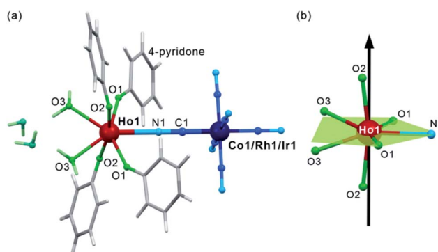
Fig. 1 The crystal structure of 1–3 presented using the structural model of 1 : the representative view of \{\text{Ho}^{\text{III}}[\text{M}^{\text{III}}(\text{CN})_6]\} ( \text{M} = \text{Co} , Rh, Ir) molecules with accompanying crystallization water (a), and the insight into the Ho III complexes with the indication of the equatorial plane of the pentagonal bipyramidal geometry (green) and the direction of their easy magnetic axis determined by the ab initio calculations (black arrow) (b).
