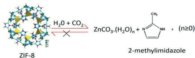
Fig. 12 Permanent collapse of ZIF-8 structure upon \text{CO}_2 adsorption in aqueous media (reprinted with permission from J. Phys. Chem. C . 2016, 120 , 13287–13294. Copyright (2016) American Chemical Society).
