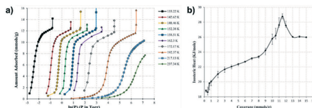
Fig. 13 a) \text{CO}_2 adsorption isotherms on ZIF-8 at a range of cryogenic temperatures and b) the isosteric heat of adsorption as a function of the surface coverage (reprinted from Russel, B. A., Migone, A. D. Microporous Mesoporous Mat. 2017, 246 , 178–185. Low-temperature adsorption study of \text{CO}_2 in ZIF-8, copyright (2017), with permission from Elsevier).
