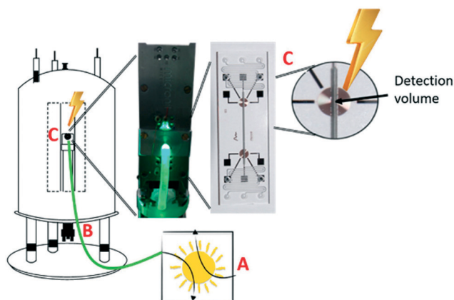
Fig. 4 Graphic representation of the assembly of nanolitre- in situ -NMR microfluidic chips. (A) UV-vis light source. (B) Non-contact-sample optical fibre. (C) Sampling zone (adapted from ref. 34 copyright 2018 American Chemical Society).
