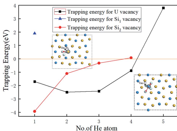
Fig. 4 The dependence of the trapping energy on the number of He atoms trapped in Vac-U, Vac-Si 1 , and Vac-Si 2 vacancies of U_3Si_5 .
