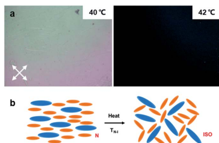
Fig. 3 (a) Thermo-optical responses of the unpolymerized LC mixture with 6% RM257. (b) The N–I phase transition of the LC mixture before polymerization.
